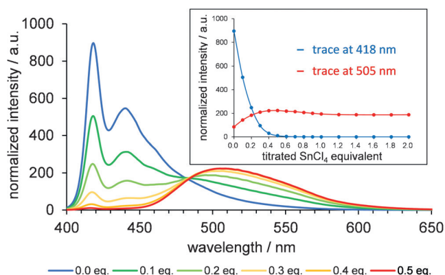
Figure 3. Changes in the emission spectra of polymer 3 upon \text{SnCl}_4 titration (excitation: 380 nm). The inset indicates emission intensity traces at 418 nm (derived from the metal-free chromophore) and 505 nm (derived from the \text{Sn}^{\text{IV}} -coordinated chromophore).
