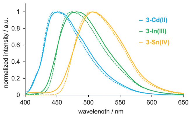
Figure 4. Emission spectra (excitation: 380 nm) of 3-Cd II (light blue), 3-In III (green), and 3-Sn IV (yellow). Dashed lines indicate spectra measured in \text{CHCl}_3 . Solid lines indicate spectra measured from solid state films.
